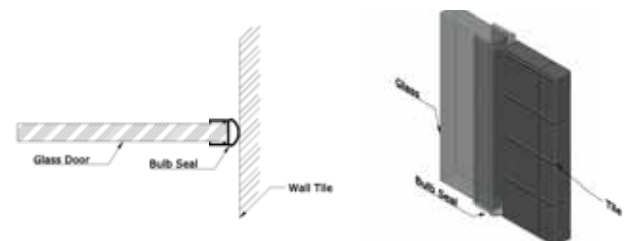
Vertical bulb seal for Active Door
