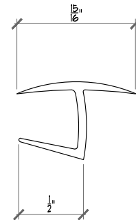
SECTION VIEW
