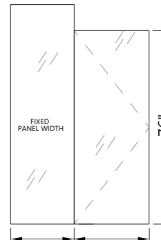
PLAN - OPTION 4
